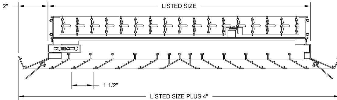
MODEL - AMD-S - SHOWN WITH OPTIONAL DEFLECTOR AND OPPOSED BLADE DAMPER
